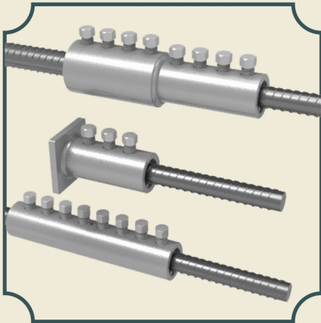
MBT Coupler
